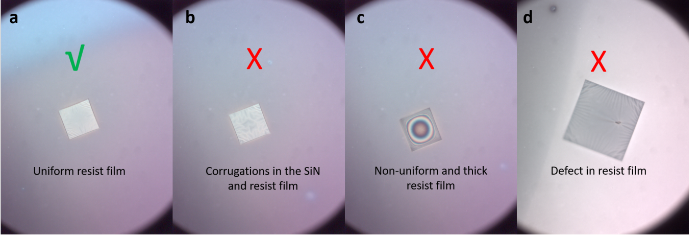
Figure 2. PMMA resist film quality after spin coating. (a) A uniform resist film. (b) Corrugations in the SiN and the resist film. (c) A non-uniform and thick resist film. (d) A defect in the resist film. Out of the 4 resist films, electron-beam lithography should only be performed with the uniform film (a).
