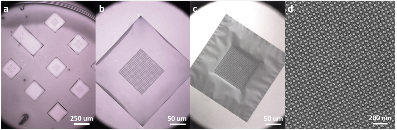
Figure 4. Mesh gratings (hole arrays) fabricated in suspended SiN membranes. (a) Optical image of the TEM grid with several mesh gratings fabricated in multiple windows. (b) Optical image of one window on the TEM grid with a large-area mesh grating. Only the supporting bars [2] can be seen, and the grating mesh is too small to be resolved. (c) The same as (b), but after coating with a 10-nm-thick aluminum film. (d) Bright-field TEM image of the fabricated mesh grating. The grating half-pitch is 50 nm.
