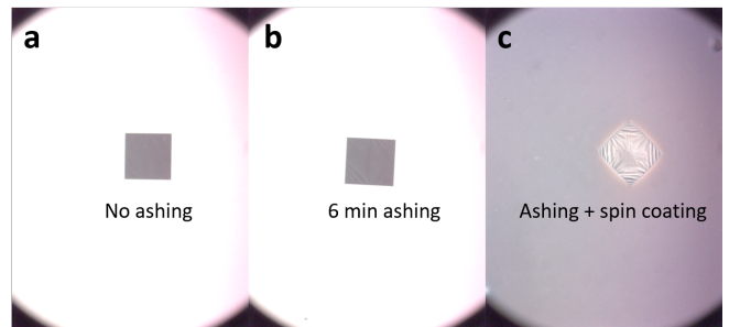
Figure 1. SiN film corrugations induced by oxygen plasma ashing. (a) SiN membrane before oxygen plasma ashing. (b) SiN membrane after 6 min oxygen plasma ashing. (c) PMMA spin-coated on SiN membrane after 6 min oxygen plasma ashing.
