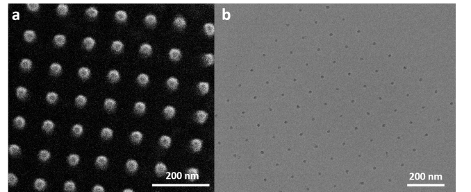
Figure 3. Aluminum nanodisks fabricated on a 5-nm-thick SiN membrane. (a) SEM image of an array of nanodisks with a large diameter created with a high exposure dose. (b) Bright-field TEM image of an array of nanodisks with a small diameter created with a low exposure dose.
